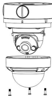
Figure 2-4 Installing the camera
