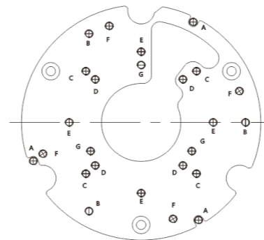
Figure 3-1 Silk-screen of installation plate
