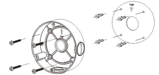
Figure 2-1 Installing the base
