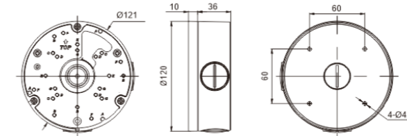
Figure 1-1 Dimensions of 0E-BBOXIP66.
