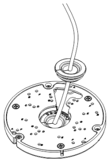
Figure 2-2 Installing the silicon plug
