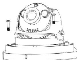
Figure 2-3 Installing the camera
